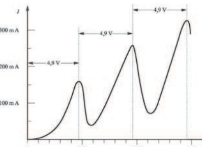
Franck-Hertzov pokus
